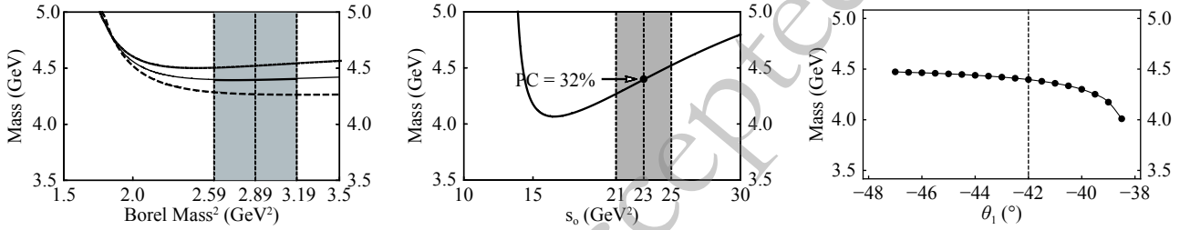
Fig. 2. Variations of M_{3/2^-} with respect to Borel mass M_B (left), threshold value s_0 (middle), and mixing angle \theta_1 (right), calculated using the current J_{\mu,3/2^-} of J^P = 3/2^- . In the left panel, the long-dashed, solid, and short-dashed curves are obtained with \theta_1 = -42^\circ and for s_0 = 21, 23 , and 25 \text{ GeV}^2 , respectively. In the middle figure, the curve is obtained with \theta_1 = -42^\circ and M_B^2 = 2.89 \text{ GeV}^2 . In the right figure, the curve is obtained for s_0 = 23 \text{ GeV}^2 and with M_B satisfying CVG=10%.
