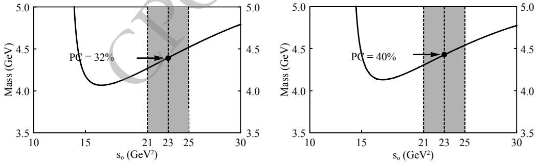
Fig. 4. Variations of M_{3/2^+} (left) and M_{5/2^-} (right) with respect to the threshold value s_0 , calculated using the current J_{\mu,3/2^+} with \theta_3 = -42^\circ and J_{\mu\nu,5/2^-} with \theta_4 = -45^\circ , respectively.
