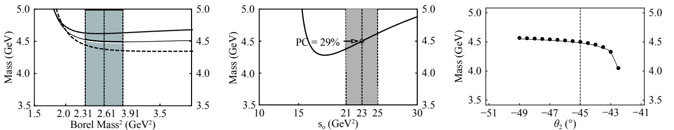
Fig. 3. Variations of M_{5/2^+} with respect to the Borel mass M_B (left), threshold value s_0 (middle), and mixing angle \theta_2 (right), calculated using the current J_{\mu\nu,5/2^+} of J^P = 5/2^+ . In the left figure, the long-dashed, solid, and short-dashed curves are obtained with \theta_2 = -45^\circ and for s_0 = 21, 23 and 25 \text{ GeV}^2 , respectively. In the middle figure, the curve is obtained with \theta_2 = -45^\circ and M_B^2 = 2.61 \text{ GeV}^2 . In the right figure, the curve is obtained for s_0 = 23 \text{ GeV}^2 and with M_B satisfying CVG=10%.
