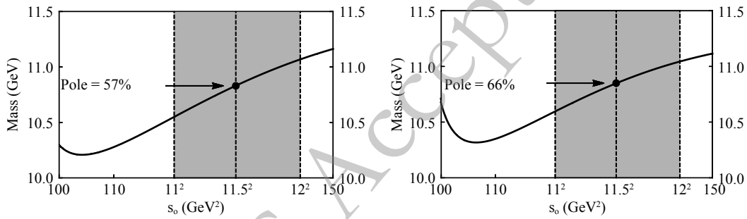
Fig. 5. Variations of M_{P_c(3/2^-)} (left) and M_{P_b(5/2^+)} (right) with respect to the threshold value s_0 , calculated using the current J_{\mu,3/2^-}^{b\bar{b}uud} with \theta_1 = -42^\circ and J_{\mu,5/2^+}^{b\bar{b}uud} with \theta_2 = -45^\circ , respectively.
